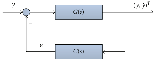
FIGURE 7: Indirect closed-loop identification setup.
