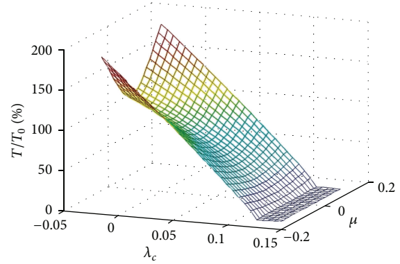
FIGURE 5: T/T_0 ratio during x - y plane movement [61].
